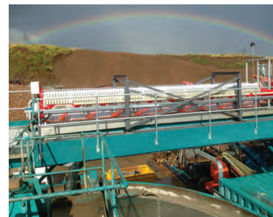
Matec 800x800 - 100 plates filter press in England
